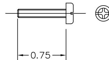
SCREW, MOUNTING
